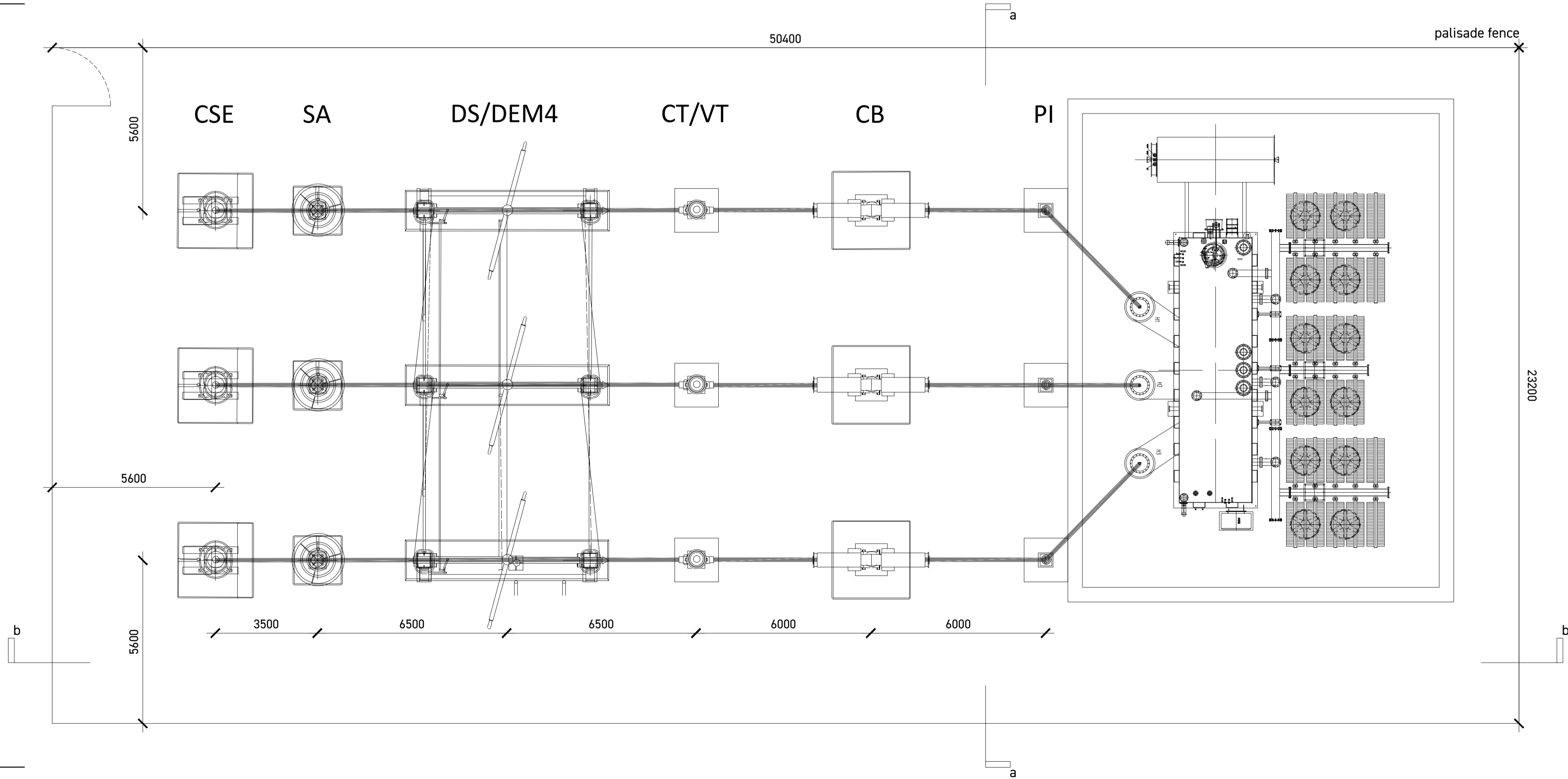
PLAN GROSS FLOOR AREA - 11685Q.M
